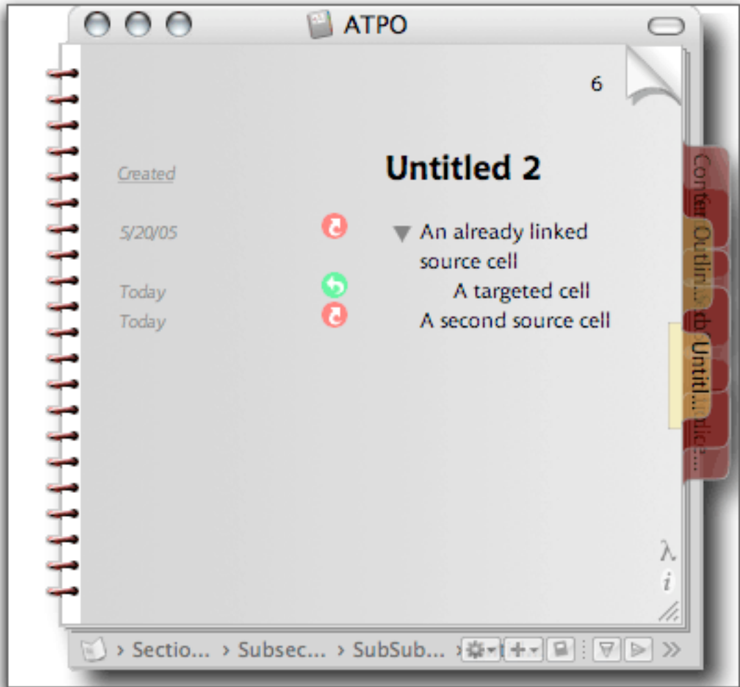
NoteBook Linking
