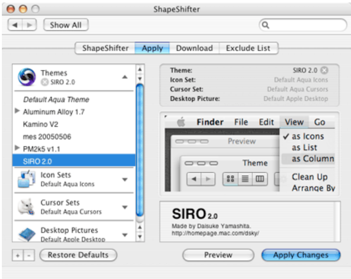
ShapeShifter
