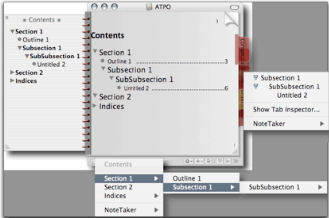
NoteBook Navigation
