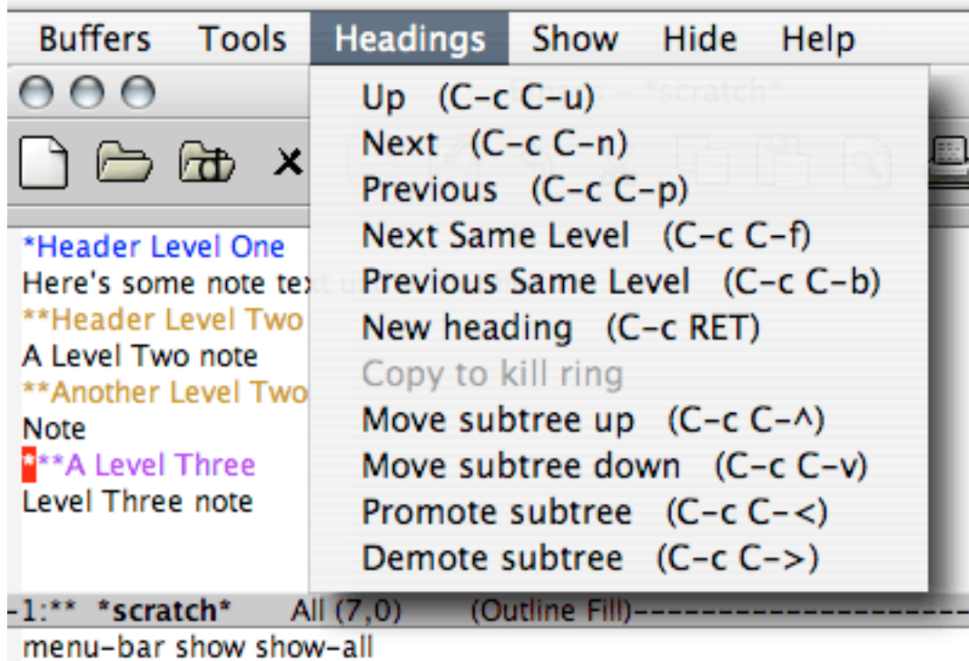
Emacs Outliner
