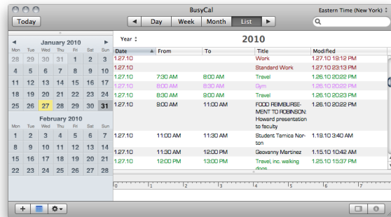
List View
